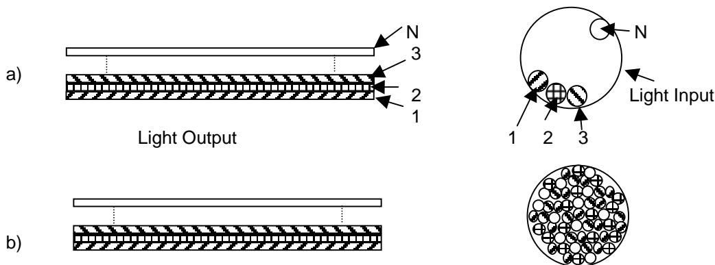
Figure 19. Possible fiber distributions or fiber randomizing for a line converter (sketch) a) coarse randomization b) fine randomization
