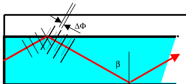
Fig. 5: Phase Shift, \Delta\Phi , after Total Reflection
