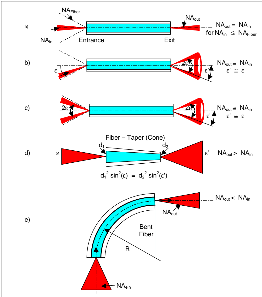
Figure 12. Relation of a fiber's radiated angle to different input angle distributions. In case b) asymmetric input coupling leads to symmetric output coupling. In d) a fiber with varying cross section (taper) changes the numerical aperture
