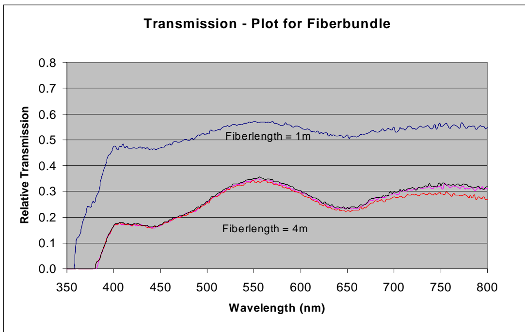
Figure 17. Fiber Bundle transmission curve ( l = 1\text{m}, 4\text{m} ; d = 3 \text{ mm} ; NA = 0.55 )
