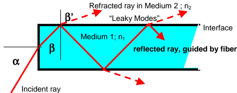
Fig 2.: Light transmission in Medium with n_1 > n_2
